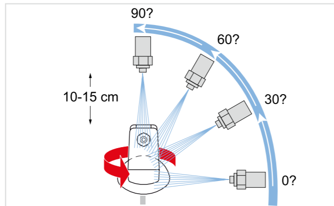
Diagram of protection rating testing IP 69K
